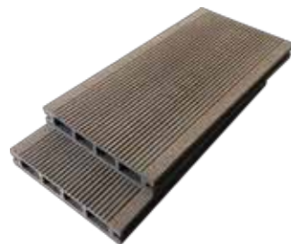
MODEL:150H25-B SIZE:150×25mm
